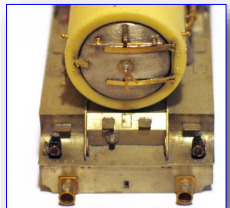
IMAGE: This image shows the front end of "British Legion". The smoke-box front and front footplate consist of more than 20 bits of brass and Nickel silver, all soldered using our own DCCconcepts solders & fluxes.
